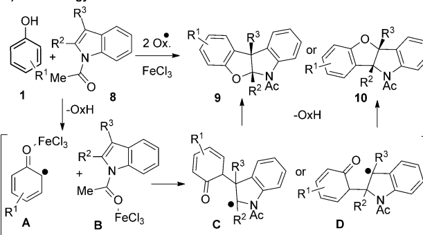
Scheme 2. Regioselective synthesis of benzofuroindolines and our radical coupling strategy.
