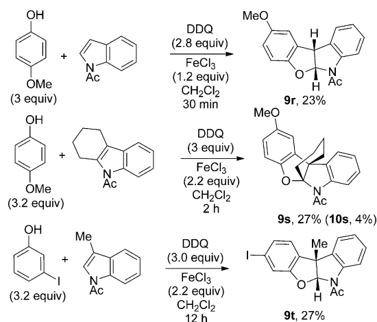
Scheme 4. Oxidative coupling between phenols and N -acetyl indoles leading to benzofuro[2,3- b ]indolines.
