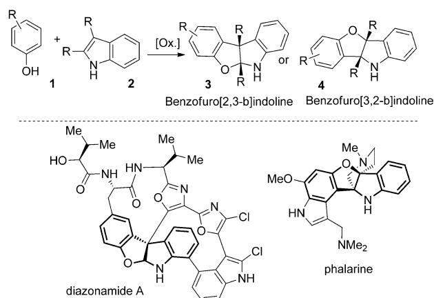
Scheme 1. Postulated biogenesis of benzofuroindolines from natural origin.
