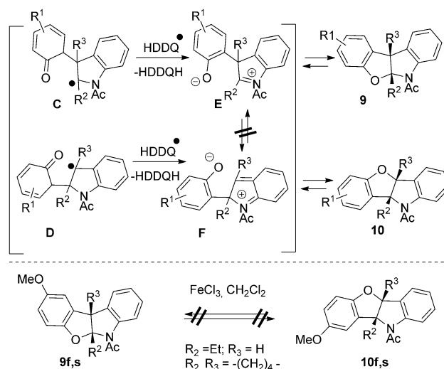
Scheme 5. Mechanistic considerations of the regioselectivity.
