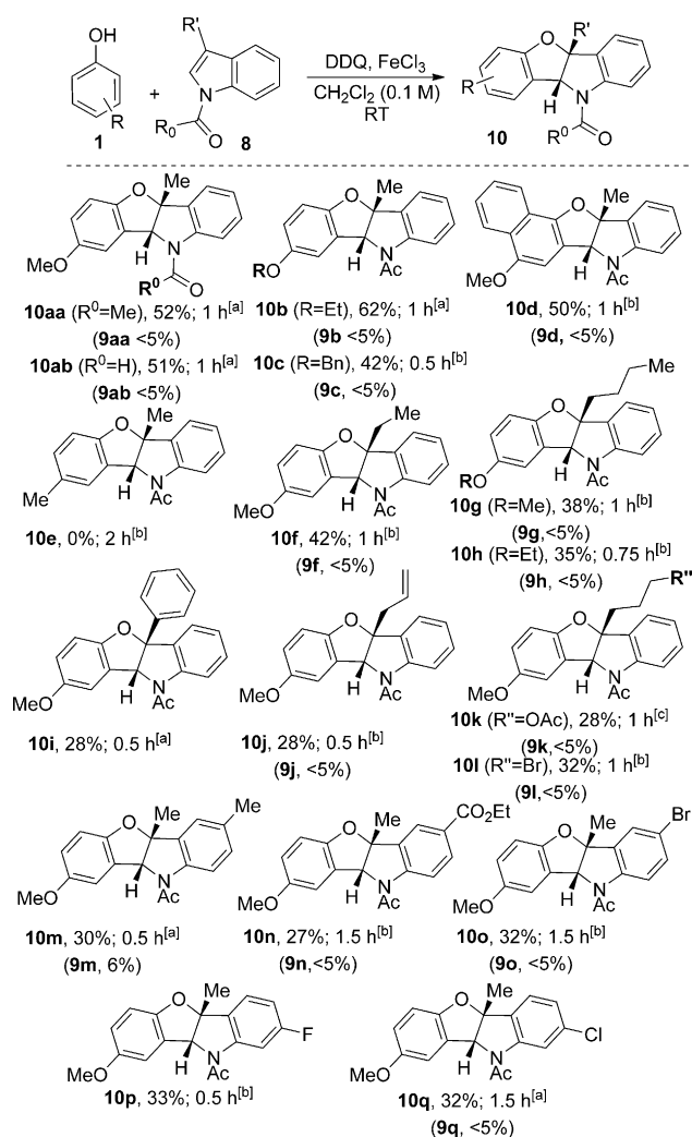
Scheme 3. Oxidative coupling between phenols and N -acetyl indoles leading to benzofuro[3,2- b ]indolines. [a] 1.5 equiv phenol, 1.5 equiv DDQ, and 1.1 equiv FeCl 3 ; [b] 3.0 equiv phenol, 3.0 equiv DDQ, and 2.2 equiv FeCl 3 ; [c] 4.0 equiv phenol, 4.2 equiv DDQ, and 2.2 equiv FeCl 3 .
